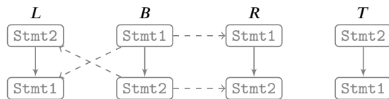
Figure 6: A swap-change merge scenario of three statement-lists ( B, L, R ) with the target T . A dashed edge between two statements indicates they are matched.
