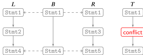
Figure 5: A conflicting merge scenario of three statement-lists ( B, L, R ) with the target T . A dashed edge between two statements indicates they are matched.
