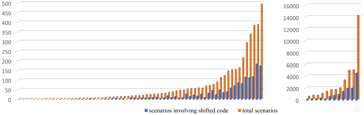
Figure 7: Distribution of shifted code in each project. The projects are sorted by their number of merge scenarios in ascending order. We split them into two subfigures according to if the number of merge scenarios is less than 500 (left) or not (right).
