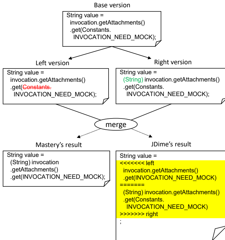
Figure 9: A merge scenario from commit 9f5cc83 of project dubbo, where an expression gets shifted. Mastery’s result is expected, while JDime’s is conflicting.
