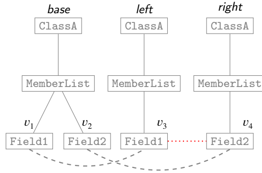
Figure 3: A merge scenario ( base , left , right ) with established mappings (dashed or dotted lines). The red dotted line shows a mapping established by comparing left and right . Assume the similarity (measured by a heuristic cost function) between Field1 and Field2 exceeds a given threshold.
