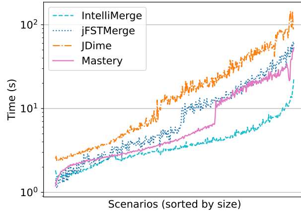
Figure 11: Time cost of merging.
