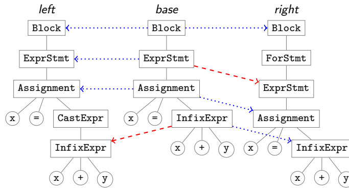
Figure 1: A merge scenario with shifted code. (Shifted mappings are depicted as dashed arrows.)
