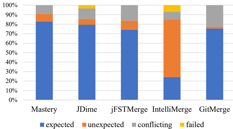
Figure 8: Distribution of the merging results.
