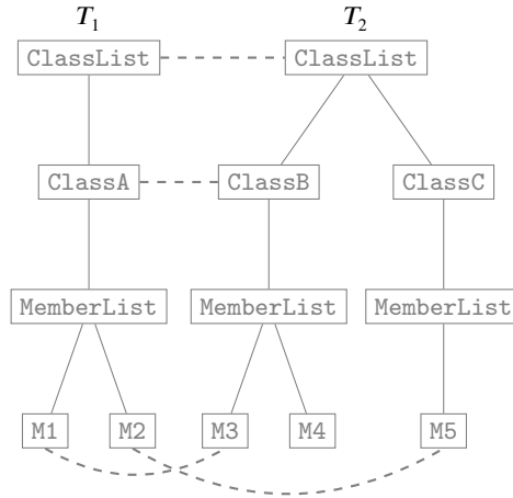
Figure 12: A non-monotone matching between T_1 and T_2 (dashed lines show mappings).
