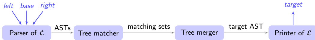
Figure 2: Workflow of our merge framework Mastery.
