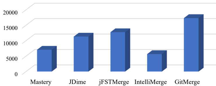
Figure 10: The numbers of conflicting blocks of the five tools.
