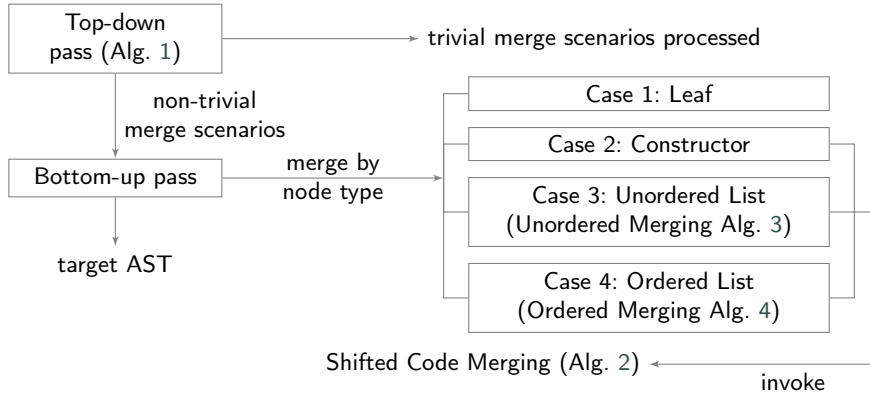
Figure 4: High-level workflow of our merge algorithm.
